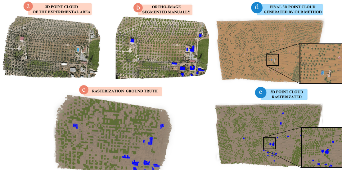
Fig. 11. The validation of the final 3D point cloud. (a) The UAV point cloud, (b) a semantic segmentation of the aerial image of the zone. On the top right (d) the procedurally generated cloud. Finally, below (c)(e) the regular classified rasterizations where standard colors are assigned by class (vegetation - green, terrain - brown, structures - blue).
