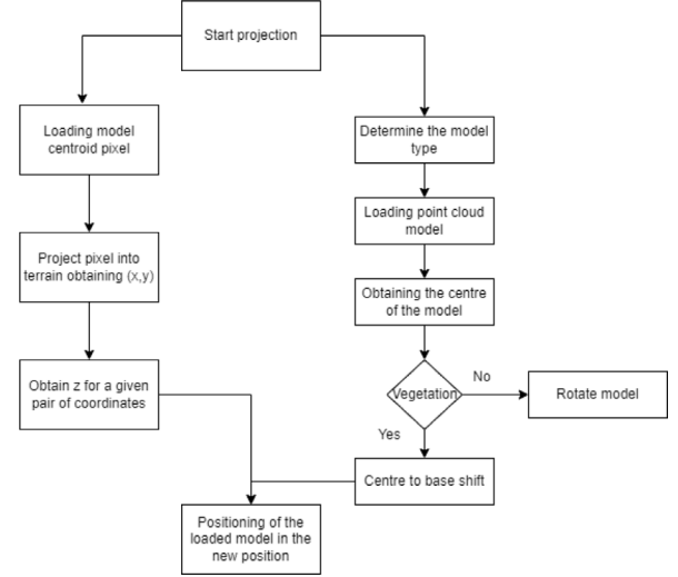
Fig. 10. Workflow for the projection of an element on the ground. The left side represents the obtaining of the central positioning coordinate, while the right side represents the transformations the model undergoes before being instantiated.
