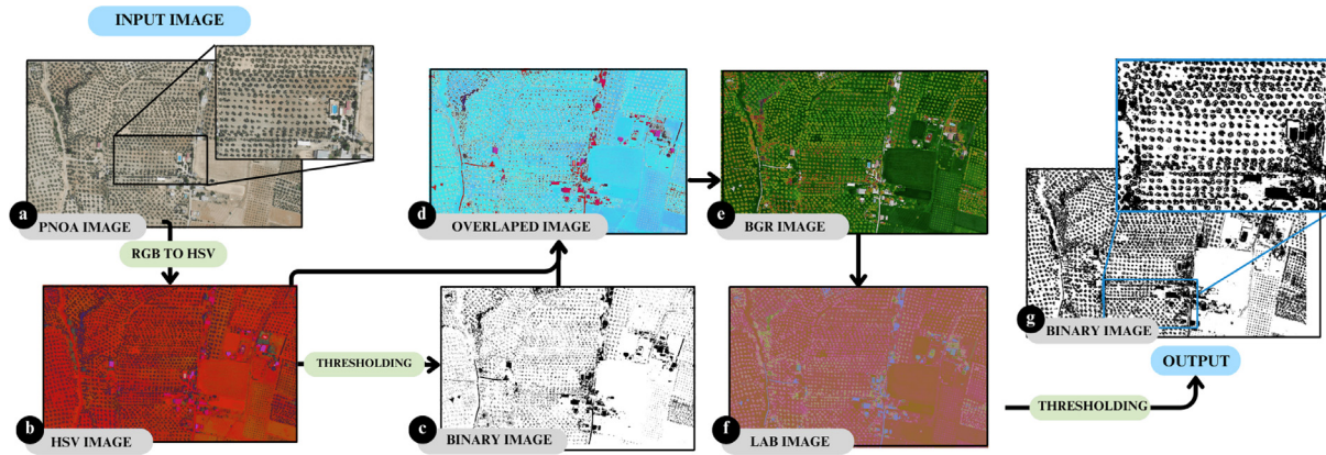
Fig. 3. The main steps of our automatic method to identify vegetation in PNOA images. As a result, the algorithm provides a binary image in which the image pixels belonging to vegetation are identified.
