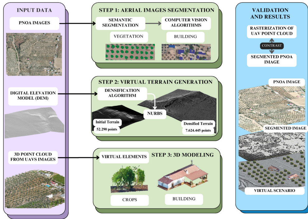
Fig. 1. An overview of the proposed workflow that summarizes the main steps of the proposed solution combines an AI-based technique for fast-forward image labeling and the generation of 3D rural scenarios.
