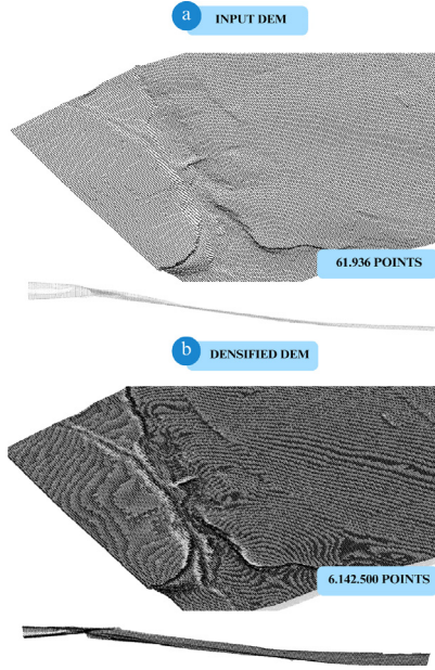
Fig. 7. The implemented densification method by applying the Non-Uniform Rational B-Splines algorithm (NURBS) to initial DEM.
