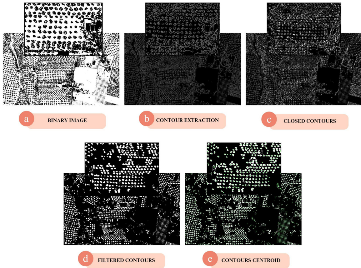
Fig. 5. Development flow of the procedure to obtain the centroid of olive trees in segmented vegetation images.
