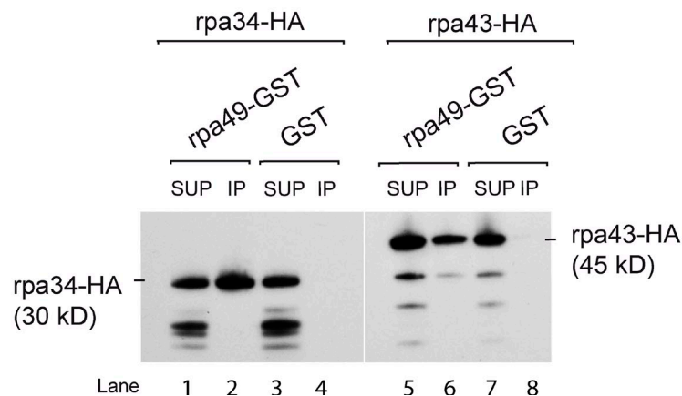
Figure 8. Two successive elongating Pol I complexes allow a contact between Rpa49 and Rpa43 subunit of adjacent molecules. (A) Frequent association of adjacent Pol I depends on Rpa49. We generated diploid cells expressing two versions of Pol I containing an Rpa190 subunit fused to either the Myc or HA tag. These tagged proteins are efficiently detected in cell extract supernatants (SUP). After formaldehyde cross-linking and extensive DNase treatment, we immunoprecipitated Pol I using anti-HA antibodies (IP). We evaluated the amount of polymerase dimers/multimers by assessing the extent of Myc-tagged Rpa190 coprecipitation. We use a strain bearing only Myc-Tag Pol I as negative control (no HA tag; lanes 1 and 4). The presence of dimers/multimers is dependent on Rpa49, as shown by lack of Myc-tagged Rpa190 coimmunoprecipitation in rpa49 deletion background ( rpa49Δ ; compare lanes 5 and 6) (B) 3D model of Pol I as determined by cryo-electron microscopy. The positions of the Pol I-specific Rpa43/Rpa14 and Rpa49/Rpa34 heterodimers are shown in purple and in green, respectively. (C) Fitting of the atomic structure of the highly homologous Pol II elongation complex (Protein Data Bank accession no. 2YU9) into the cryo-electron microscopy structure of RNA Pol I. The transcribed DNA is shown in red, and the 10-subunit core Pol II is shown in blue.
