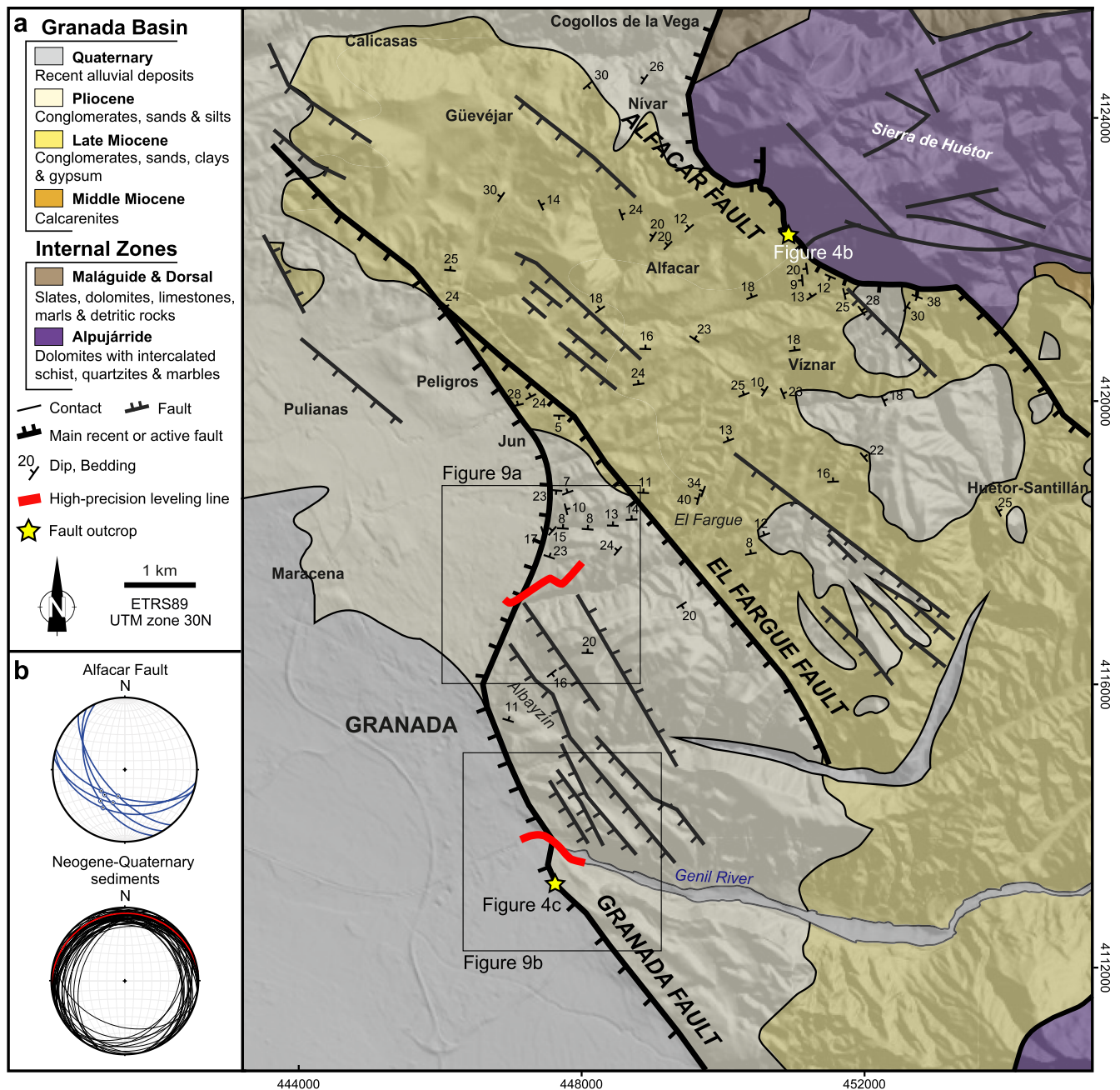
Figure 3. (a) Detailed geological map of the northeastern edge of the Granada Basin, including the main tectonic structures, modified from Galindo-Zaldívar et al. (2015). Location of outcrops illustrated in Figure 4 and high-precision leveling lines are indicated. The location of this area is given in Figure 2. (b) Stereonets (Schmidt net, lower hemisphere) of dip/dip directions of the Alfacar fault and the Neogene-Quaternary sediments.
