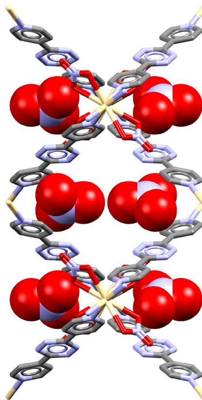
Fig. 26. Fragment of the LIWFEE crystal structure (catena-[bis(3,6-di(pyridin-4-yl)-1,2,4,5-tetrazine)-dinitrato-cadmium(ii) tetrakis(thiourea)-cadmium(ii) dinitrate]), featuring parallel stacks of strongly interacting s -tetrazine rings and nitrate anions. Angle between \text{NO}_3^- and s -tetrazine mean planes: 7.1^\circ [162].
