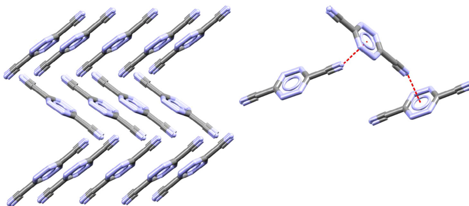
Fig. 35. Structural features of JOYXEC: overall crystal packing (a) and details of lone pair- \pi contacts (b) (N...centroid 2.83 Å, offset 0.20 Å, angle 85.9°) [168].
