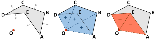
FIGURE 4. A 2D simplicial covering of a n-sided polygon. A triangle is generated for every segment, and has a sign for the covering that depends on the orientation of the segment with respect to O . In this example the simplicial covering of the polygon is composed of 3 positive triangles and 2 negative triangles.
