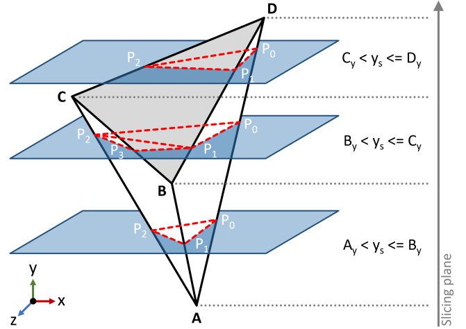
FIGURE 6. Slicing planes for rasterizing a tetrahedron.
