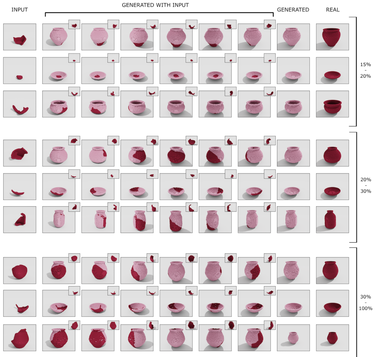
Figure 3: Qualitative examples for visual comparison of completed samples by our proposed method and the ground truth (real voxelized models). Each batch of examples shows the completion model started from different sizes of initial fragments (dark pink), and the completed ceramics (light pink) in different views.
