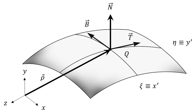
FIGURE 1 Schematic illustration showing the components of the Frenet trihedral for an arbitrary point over a generic non-flat surface 24
