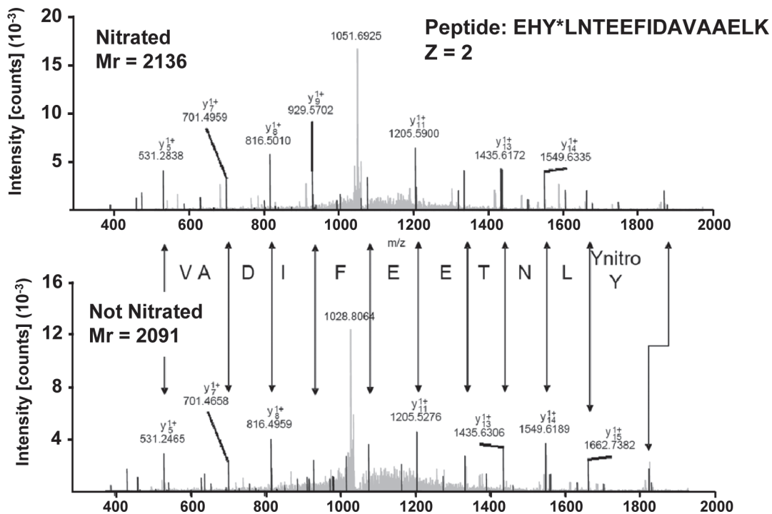
Fig. 6. Comparison of the nitrated (top) and unmodified (bottom) MS/MS spectra of the identified peptide (EHYLNTEEFIDAVAAELK) from the cytosolic pea NADP-isocitrate dehydrogenase.
