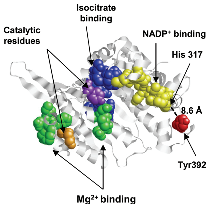
Fig. 7. Three-dimensional model of cytosolic NADP-isocitrate dehydrogenase showing Tyr392 (red) and its potential interactions. Conserved residues implicated in the binding of Mg^{2+} (green), isocitrate (blue), and NADP (yellow); catalytic residues are shown as purple or orange. The NADP-binding site includes Lys376 and His317 and is at 8.6 Å of the nitrated Tyr392 (this figure is available in colour at JXB online).
