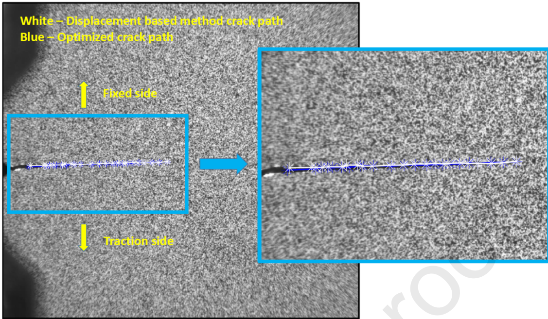
Figure 14: Crack paths superimposed over the speckle image
