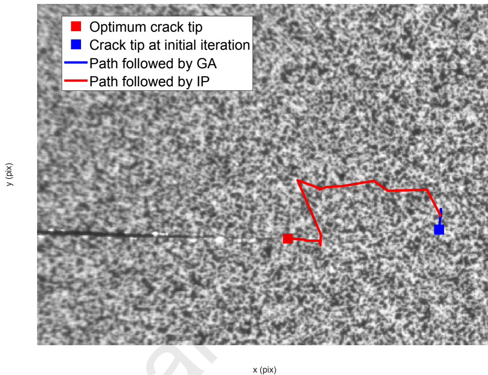
Figure 11: Illustration of the final optimum crack tip position (red square), the crack tip position at the first iteration (blue square), and paths followed by the optimization algorithms (blue GA and red IP) superimposed on the speckle image. Crack length of 7.75 mm.
