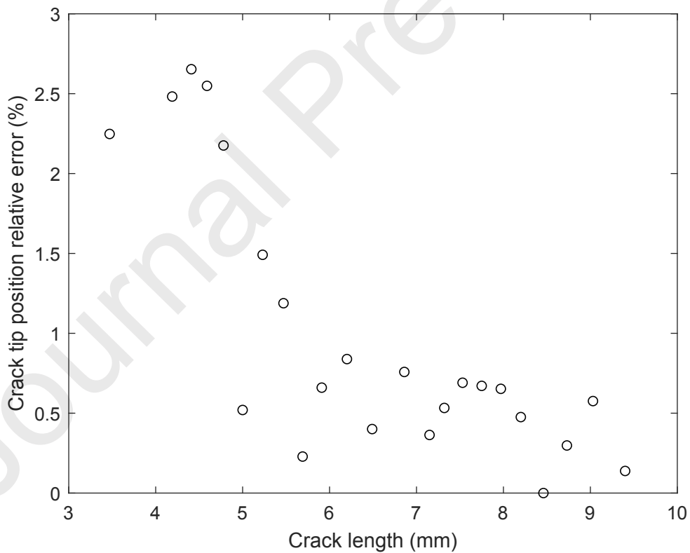
Figure 15: Relative crack tip position difference between the hybrid optimisation and the displacement intersection methods.
