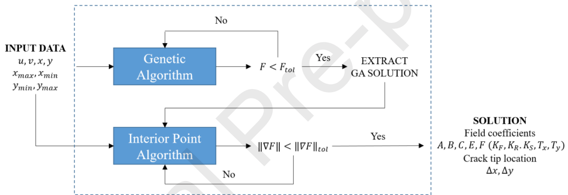
Figure 6: Hybrid optimisation scheme.
