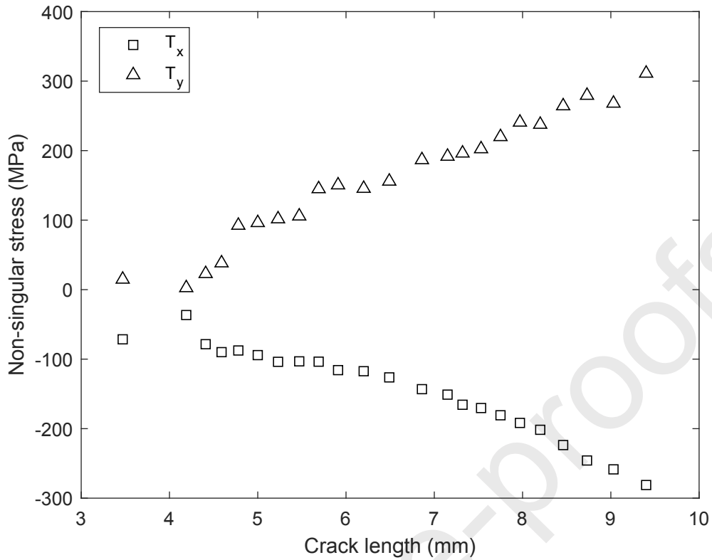
Figure 16: Non-singular stresses along x and y axes in function of crack length
