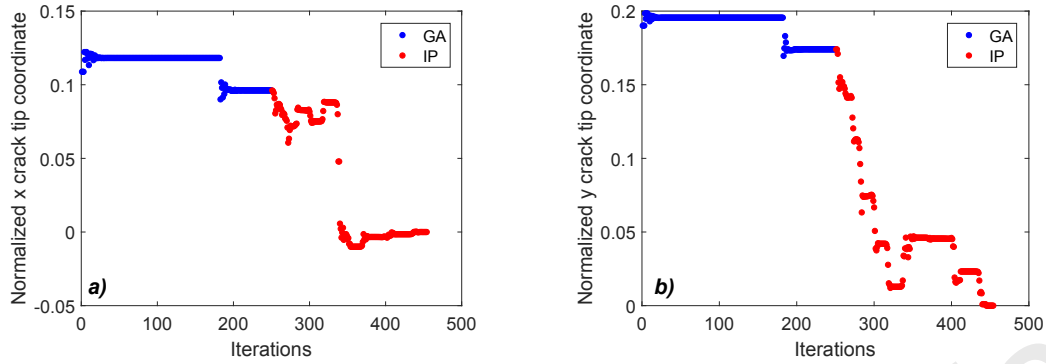
Figure 12: Changes in the x and y crack tip coordinates during the iterative process, normalised as the ratio of the distance between their x and y distances and the optimum crack tip position divided by the crack length. A value of zero corresponds with the normalised optimum crack tip position during the optimisation process. a) x -coordinate and b) y -coordinate.
