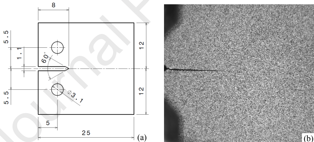
Figure 1. (a) Dimensions of the CT specimen (mm). (b) Speckle pattern sprayed onto the specimen surface for the DIC work.
