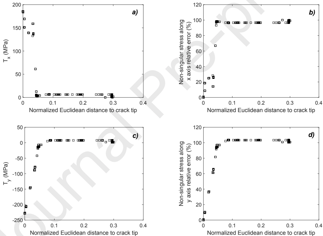
Figure 10: Variation of non-singular stresses with the normalised Euclidean distance to the crack tip for a crack length of 7.75 mm. Crack tip distance normalised by crack length. a) T_x , b) T_x relative error, c) T_y and d) T_y relative error.
