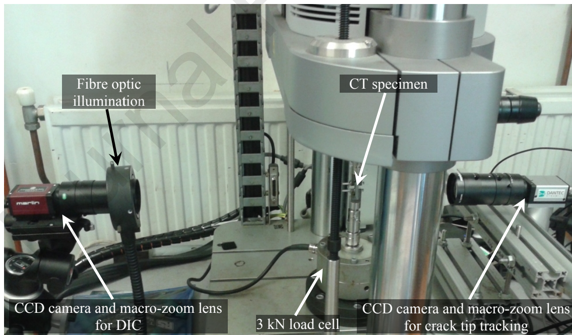
Figure 2. Experimental set-up used in the fatigue testing and for data acquisition.
