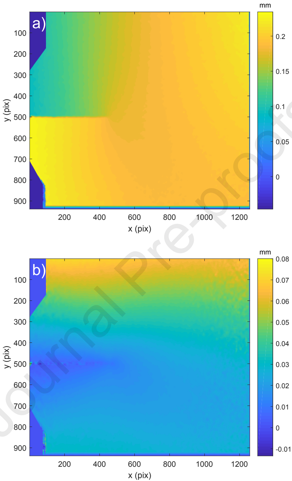
Figure 3. (a) Vertical and (b) horizontal displacement maps measured with DIC for a 9.40 mm crack at a load of 750 N.
