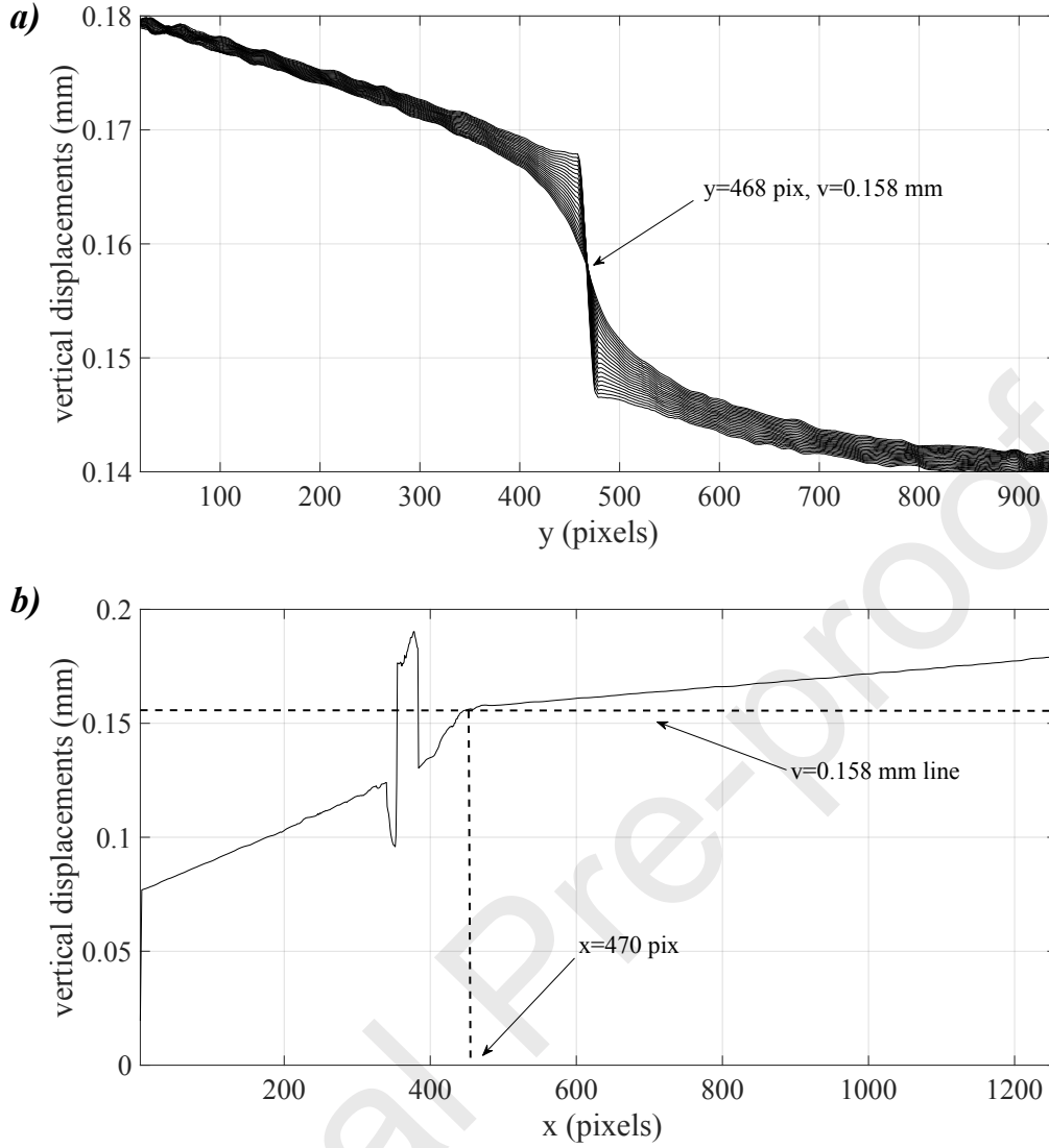
Figure 7. Plots showing the methodology used to identify the position of the crack tip in the y (a) and x (b) directions.
