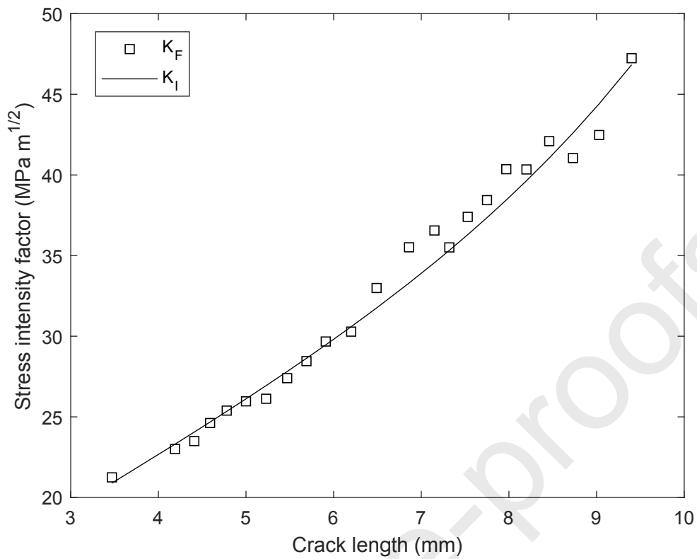
Figure 13: Experimentally determined CJP driving force, K_F , and standard Mode I stress intensity factor versus crack length at maximum load.
