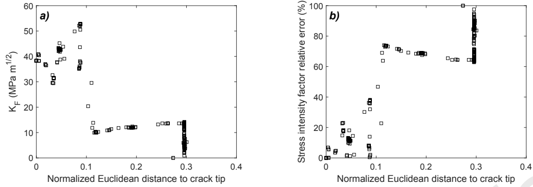
Figure 9: Variation in opening mode SIF with the normalised Euclidean distance to the crack tip for a crack length of 7.75 mm. Crack tip distance normalised by crack length. a) K_F and b) Relative error in terms of K_F
