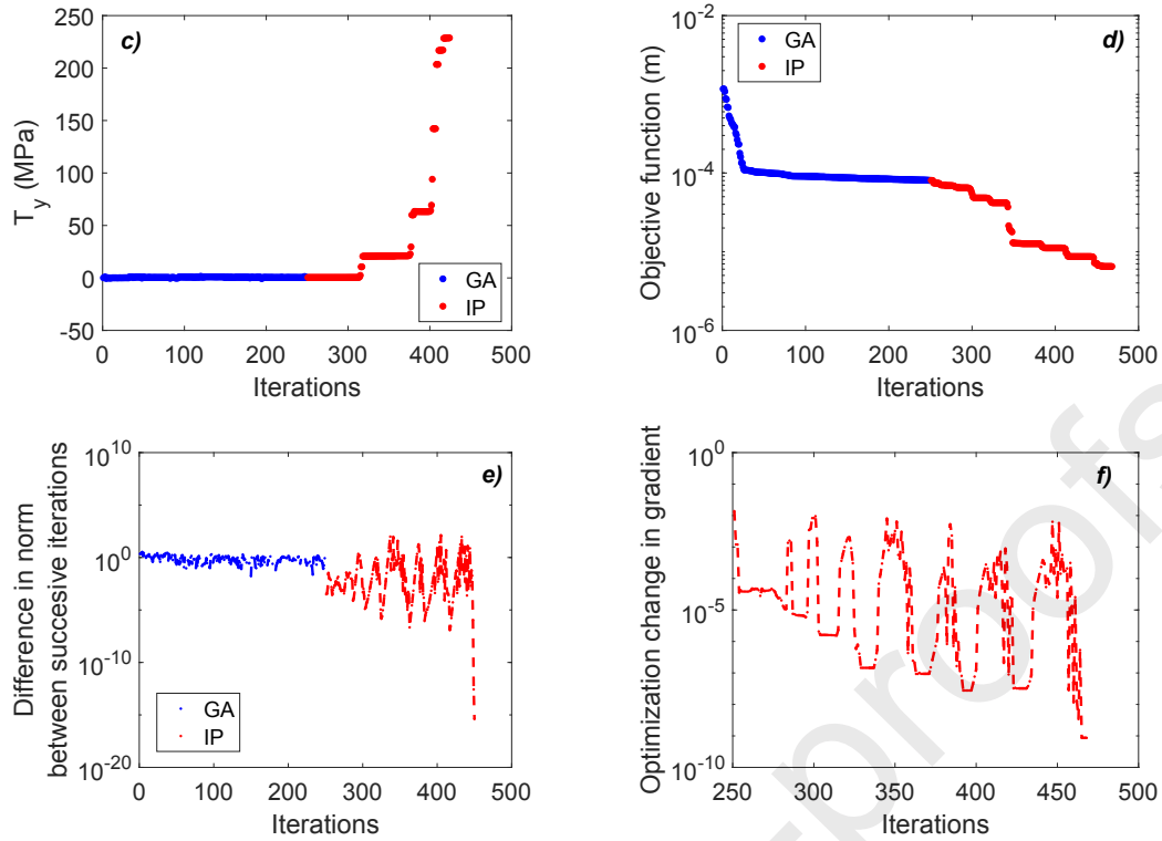
Figure 8: The changes in specific parameters observed during the optimisation process for a crack length of 7.75 mm. a) CJP opening mode SIF K_F , b) and c) Non-singular stresses T_x and T_y , d) Objective function e) Difference in norm between successive iterations and f) Optimisation change in gradient (only computed for the gradient-based method)
