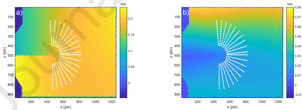
Figure 4: Annular mesh superimposed on a) vertical and b) horizontal displacement maps for a crack length of 9.4 mm at maximum load.
