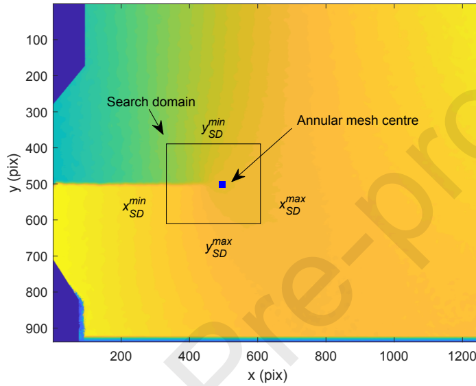
Figure 5: Search domain in the vertical component of the displacement field.
