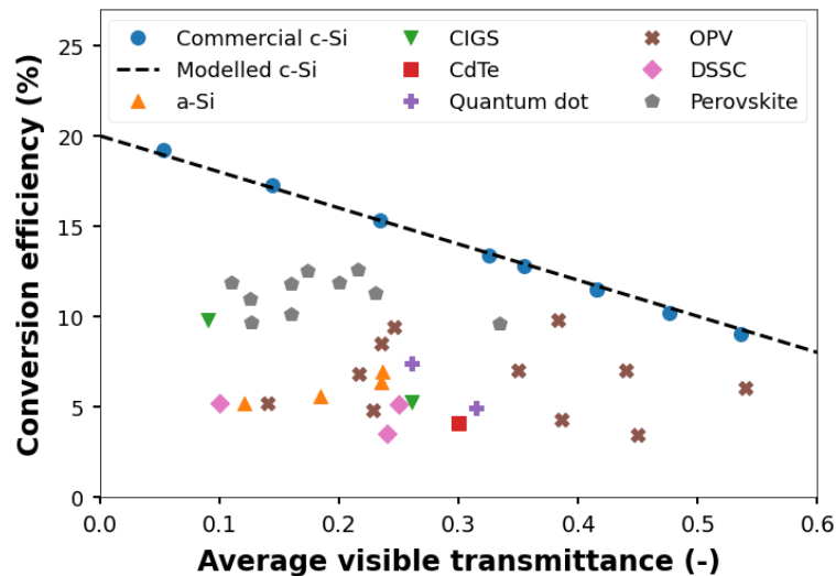
Figure 1. Conversion efficiency as a function of the average visible transmittance of different PV technology taken from [45]. The efficiency of commercial c-Si technology from BISOL Group, d.o.o. has been also included (Bisol Lumina series: https://www.bisol.com/pv-modules ). The modelling efficiency as a function of transparency of c-Si technology using the methodology proposed in this work is also shown for validation purposes.
