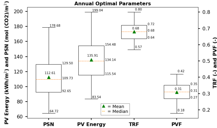
Figure 10. Mean, median, maximum, minimum and percentiles 25 and 75 (represented by the boxplots) of the optimal transparency factor (TRF), photosynthetic rate (PSN), photovoltaic active factor (PVF) and PV energy harvested considering the four locations under study.
