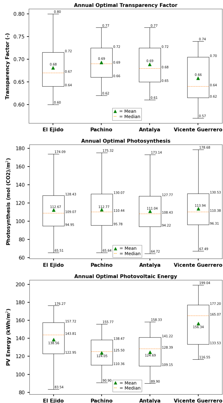
Figure 9. Mean, median, maximum, minimum and percentiles 25 and 75 (represented by the boxplots) of the annual optimal transparency factor (TRF), photosynthetic rate (PSN), and PV energy harvested for each location.
