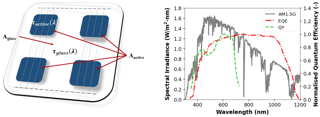
Figure 3. Left: scheme of a semi-transparent PV module composed of a transparent and a PV active area. Right: standard ASTM G173-03 global spectrum (U.S Standard Atmosphere 1976, S&F rural aerosol model, aerosol optical depth at 500 nm = 0.084 and water vapour = 1.42cm) [48], typical quantum yield (QY) of the crops [49] (with an absorption band between 400 and 700 nm approximately) and external quantum efficiency (EQE) of c-Si [50] (with an absorption band between 400 and 1100 nm approximately).
