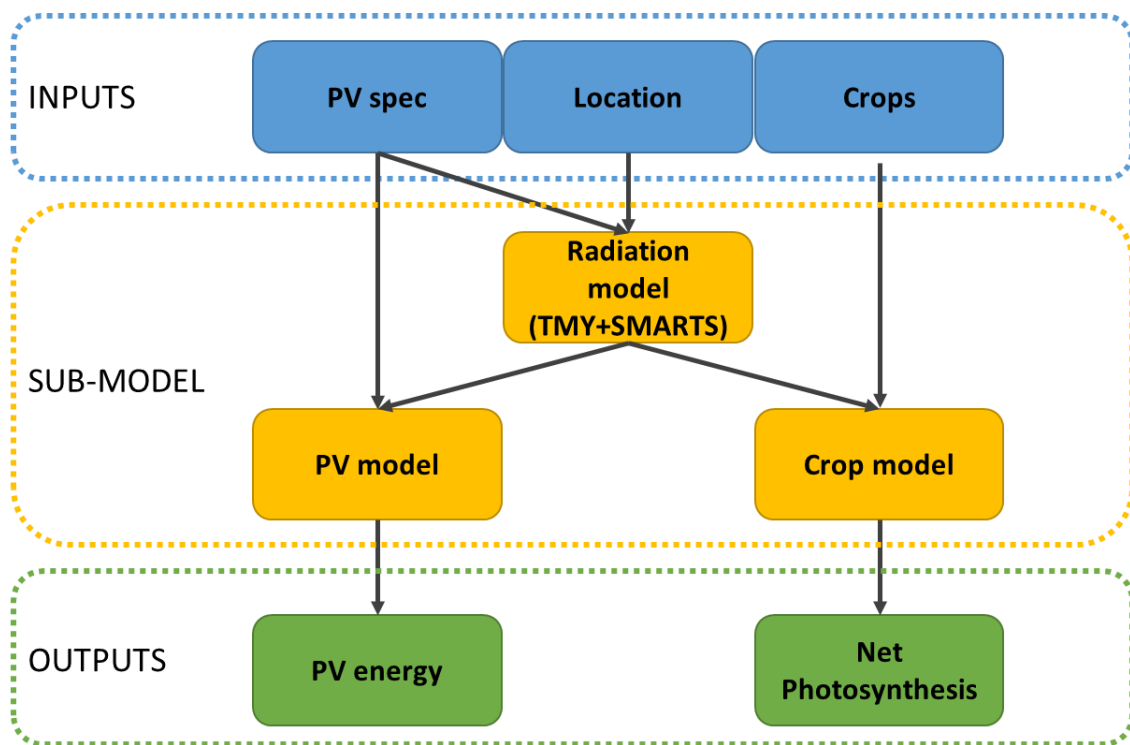
Figure 2. Flow chart of the model of semi-transparent PV integrated on greenhouses.
