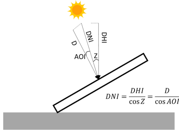
Figure 5. Scheme to explain the formulation of equation (4). Note that the DHI is the projection of the DNI on the vertical axis according to the Z angle, and the D is the projection of the DNI on the perpendicular axis of the module surface according to the AOI .
