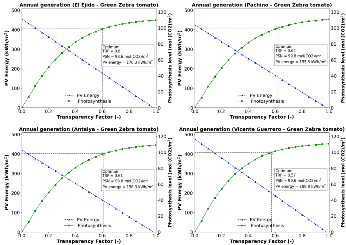
Figure 7. Relationship between the PV energy and PSN as a function of the transparency of the modules for the Green Zebra Tomato for the four selected locations.
