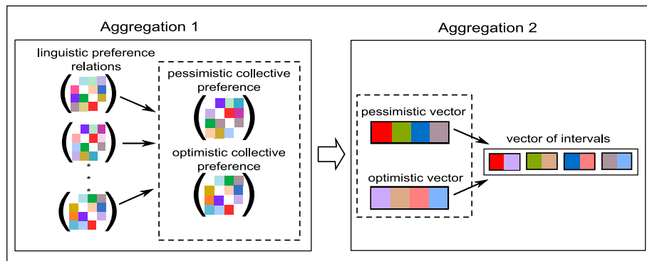
Fig. 6. Scheme of the aggregation process.
