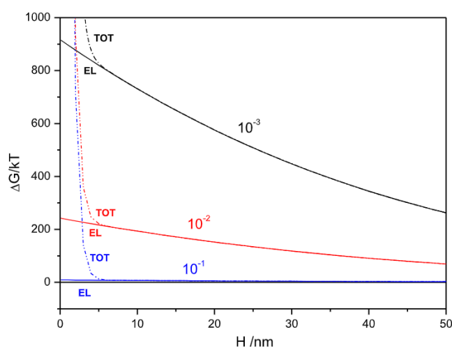
Fig. 7. Component of total energy interaction and electrical components for three ionic strength of Na + (10 -1 , 10 -2 and 10 -3 M) at natural pH for line C2C12.
