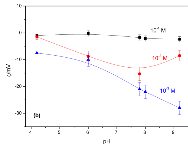
Fig. 3. Dependence of the zeta potential of cells for three ionic strength of \text{Na}^+ ( 10^{-1} , 10^{-2} , and 10^{-3} M) as a function of pH of the liquid phase: (a) cell line C2C12 and (b) breast tumour cells.
