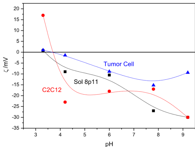
Fig. 2. Dependence of the zeta potential of the two normal cell lines and breast tumour cells at ionic strength 10^{-2} M of \text{Na}^+ , as a function of the pH of the liquid phase.
