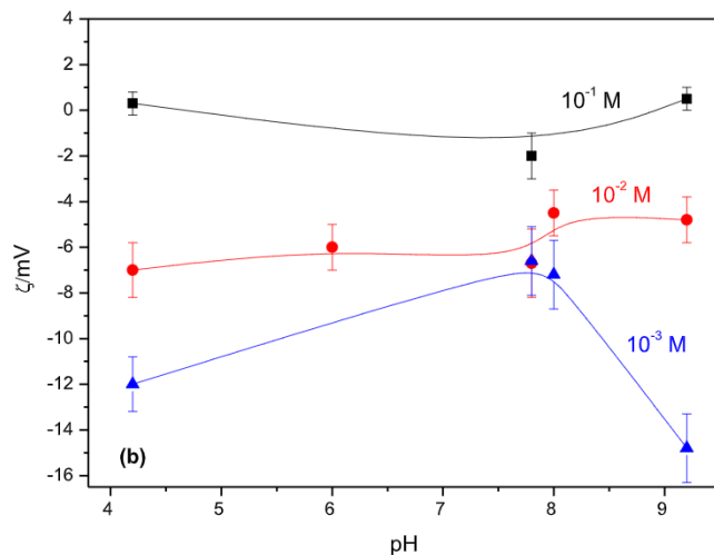
Fig. 4. Dependence of the zeta potential of cells for three ionic strength of \text{Ca}^{++} ( 10^{-1} , 10^{-2} , and 10^{-3} M) as a function of the pH of the liquid phase: (a) cell line C2C12 and (b) breast tumour cells.
