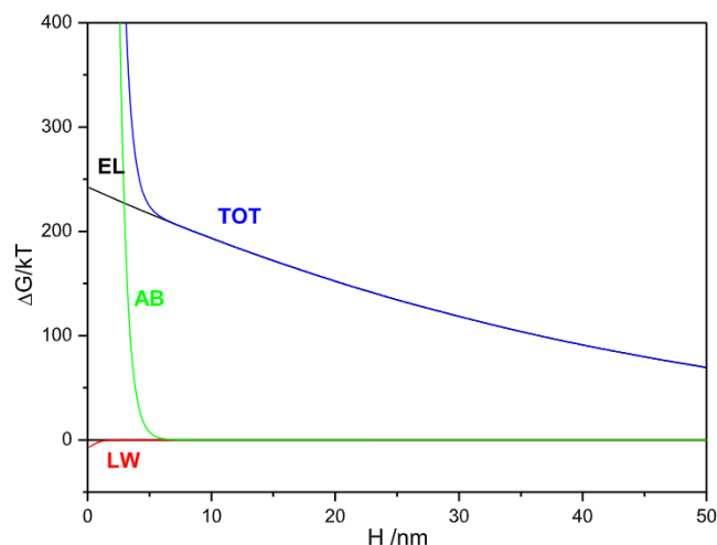
Fig. 6. Component of total interaction energy for normal cells (C2C12) at natural pH and 10 -2 M of NaCl.
