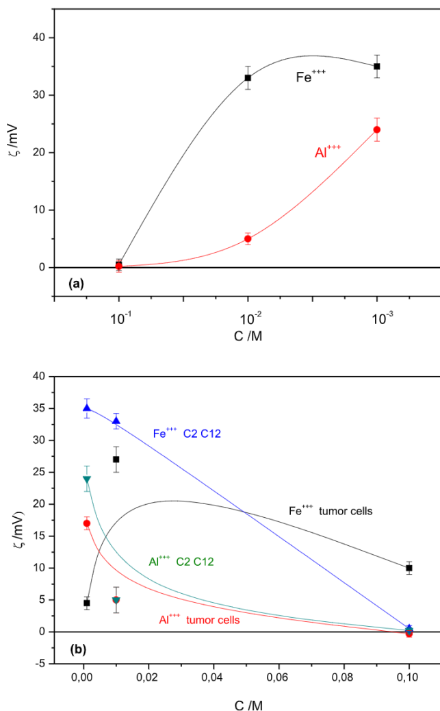
Fig. 5. Dependence of the zeta potential of cells for three ionic strengths of trivalent ions at pH≈4: (a) cell line C2C12 and (b) breast tumour cells versus normal cells.
