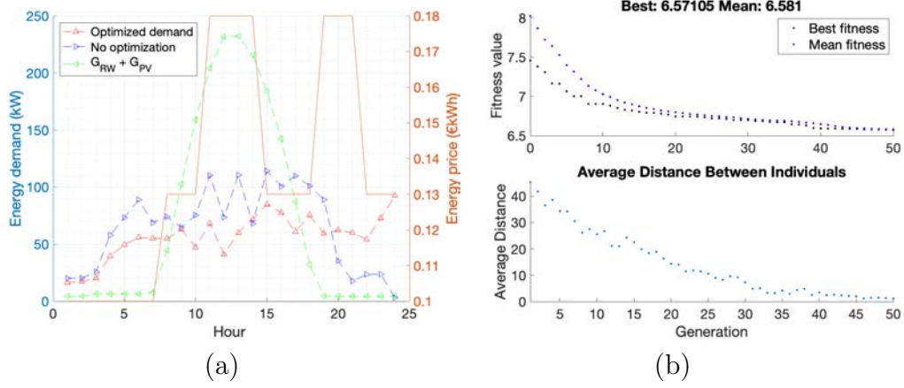
Figure 10: CASE1. Results obtained for the optimization of controllable appliances by reducing energy cost and reducing consumption peaks (a); number of needed iterations for the best mean optimized solution (b).
