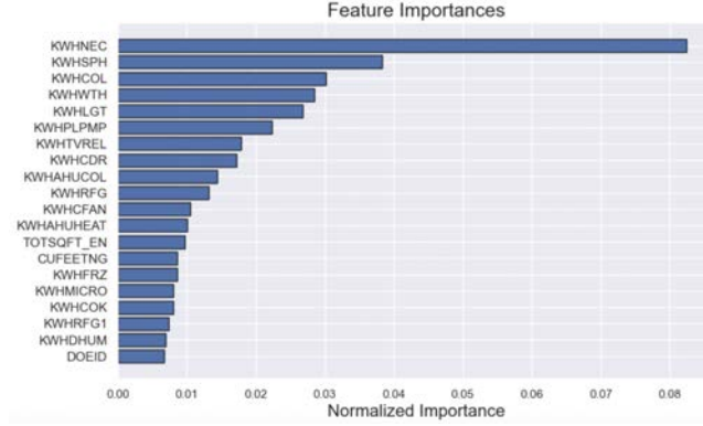
Figure 8: Variable importance scores of appliance energy consumption.
