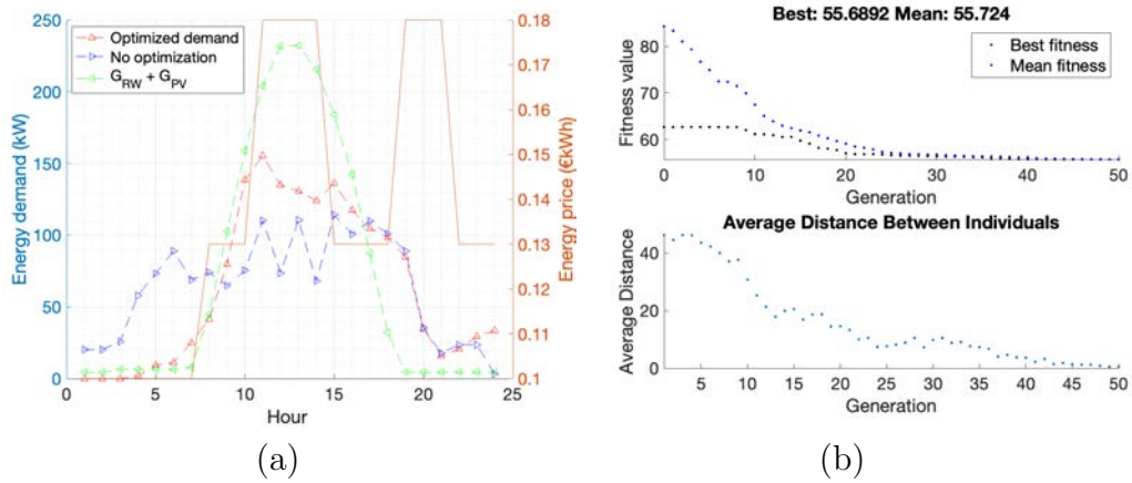
Figure 11: CASE2. Results obtained for the optimization of controllable appliances by maximizing the renewable sources and reducing consumption peaks (a); number of needed iterations for the best mean optimized solution (b).
