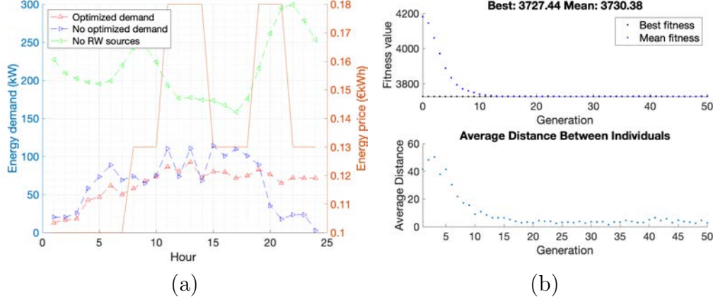
Figure 12: CASE3. Results obtained for the optimization of controllable appliances by maximizing the non renewable sources and reducing consumption peaks (a); number of needed iterations for the best mean optimized solution (b).
