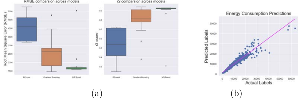
Figure 9: Tuned mode RMSE and R^2 comparison across three model for controllable loads (a); and predicted loads with higher importance in energy consumption (b)
