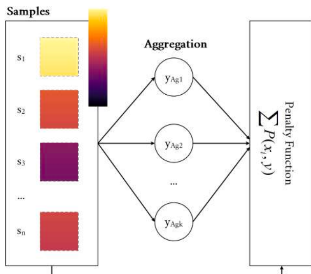
Fig. 10. Overview of a penalty function that receives as input the original thermal measurements as well as the values aggregated by different operators, in order to measure the error from samples to the aggregation.
