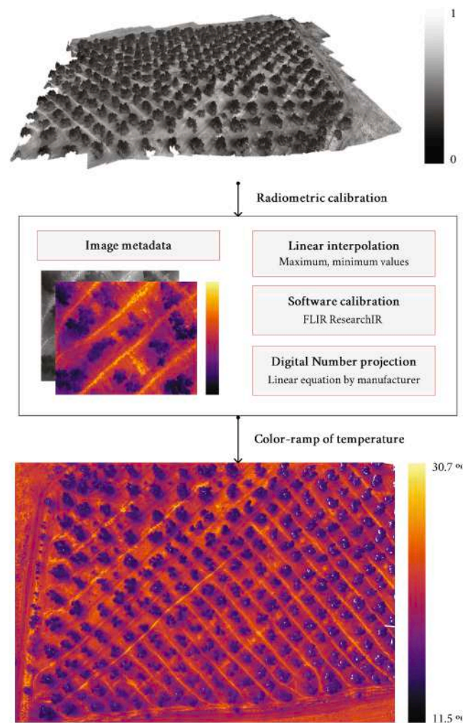
Fig. 11. Scheme of a radiometric calibration procedure. Different methods are depicted here to extract the temperature of a thermal image.
