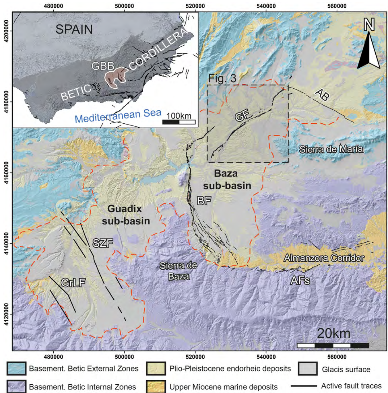
Fig. 1. Geological map of the Guadix-Baza Basin (GBB, red dashed line) and its main active structures. BF: Baza Fault, GF: Galera Fault, AFs: Almanzora Faults, AB: Alfahuara-Botardo structure, SZF: Solana de Zamborino Faults, and GrLF: Graena-Lugros Fault. The inset shows the location of the Guadix-Baza Basin in south-central Spain. DEM source: Spanish Centre of Geographical Information (CNIG, https://centrodedescargas.cnig.es/CentroDescargas/index.jsp ).
