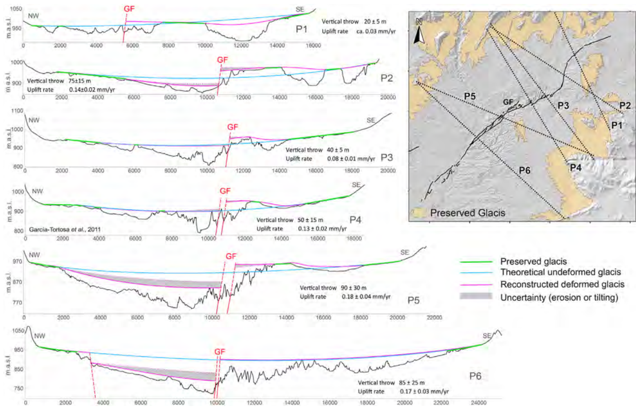
Fig. 9. Glacis surface analysis. Topographic profiles showing the theoretical uneroded and undeformed glacia (top basin surface) (blue line) and the reconstructed deformed glacia (pink line). The dotted pink line with the grey shaded area represents the uncertainty derived from possible glacia erosion. The position of the profiles is indicated in the inset map.
