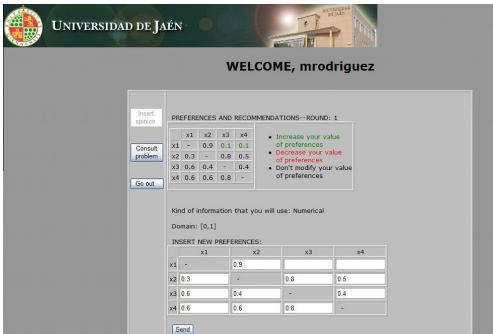
Fig. 11. The employee e_1 , receives some recommendations.
