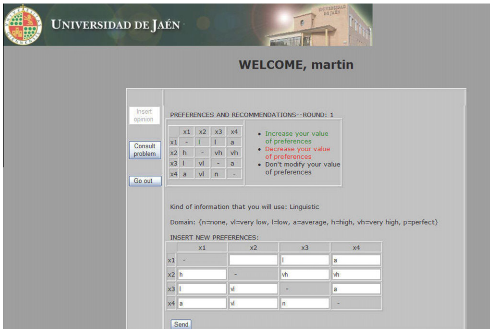
Fig. 8. A decision maker who provided his/her assessments by using linguistic terms, receives some recommendations.
