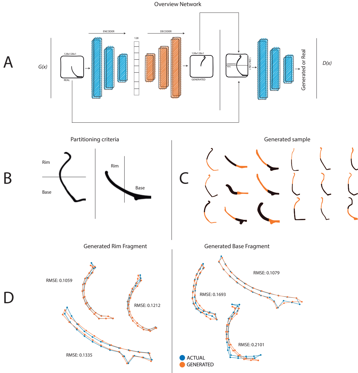
Figure 1. Overview of the proposed approach. A IberiGAN architecture. The G(x) generator is based on an encoder-decoder architecture. Upon receiving a fragment of pottery, the encoder transforms it into a vector and then the decoder generates the missing or unknown fragment. The discriminator D(x) receives the complete profile to determine if it is true or false. B Criteria for profile partitioning into rim and base of profiles. C Examples of IberiGAN generated samples from fragments for both open and closed shapes (shown in lighter color). D Semi-landmark analysis and RMSE values as comparing actual and artificially generated samples.
