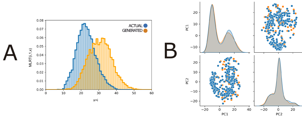
Figure 3. A GS distribution of the real (blue) and generated (orange) data set. For more information about the GS metric see section Materials and Methods: Evaluation metrics. B PCA comparison on the full real dataset and randomly generated 1200 samples.
