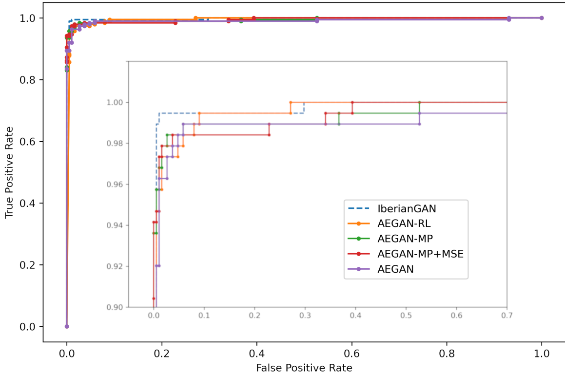
Figure S1. Receiver Operator Characteristic (ROC) curves using different generative approaches. The Area Under the ROC Curve of each method is IberianGAN: AUC_{ROC} = 0.998 , AEGAN-RL, AEGAN-MP, AEGAN-MP+MSE: AUC_{ROC} = 0.994 and AEGAN: AUC_{ROC} = 0.991 .
