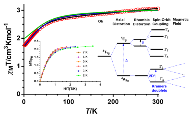
Figure 6. Temperature dependence of \chi_M T for compound 5 (red circles). Solid lines represent the best fit to equations 1 (black line) and 2 (blue line). The solid green line corresponds to the ab initio calculated \chi_M T vs. T plot. M vs. H/T isotherms (insert left) and qualitative energy splitting of the 4T_{1g} term in Oh symmetry by axial compression and rhombic distortion, SO and Zeeman effect (right). Solid lines in the reduced magnetization plot represent the best fit to equation 1.
