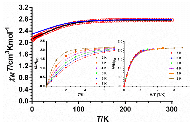
Figure 5. Temperature dependence of \chi_M T for compound 2 (red circles). Field dependence of magnetization at the indicated temperatures (insert left) and M vs H/T isotherms (insert right). Solid lines represent the best fit to equation 1 with the parameters indicated in Table 1. The blue solid line in the \chi_M T vs. T plot represents the ab initio calculated curve scaled by a factor of 0.9.
