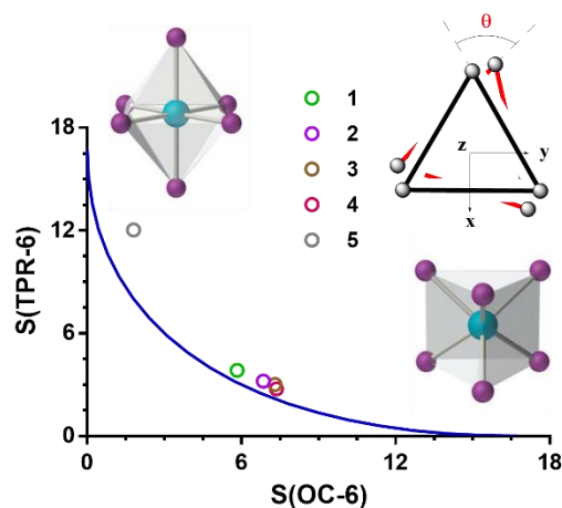
Figure 3:- Octahedron-trigonal prism shape map showing the Bailar pathway (blue line) and the experimental data (circles). Bailar twist angle ( \theta ) is also displayed (insert up right).
