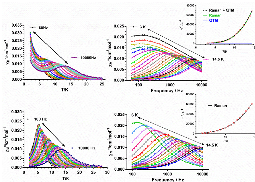
Figure 13.- Temperature dependence of \chi_M'' at different frequencies for 3' at zero field (top left) and at 0.12 T (bottom left) and frequency dependence of the relaxation time \tau at different temperatures for complex 3' at zero field (top right) and at 0.12 T (bottom right). The dotted black line represents the best fit of the experimental data to a combination of Raman and QTM processes, whereas the green and blue lines represent the Raman and QTM contribution to the magnetic relaxation, respectively (insert top right), and to a Raman process (insert bottom right).
