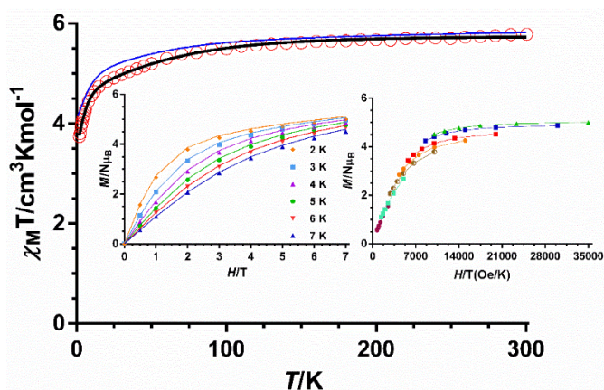
Figure 4. Temperature dependence of \chi_M T for compound 1 (red circles). Field dependence of magnetization at the indicated temperatures (insert left) and M vs H/T isotherms (insert right). Solid lines represent the best fit to equation 1 with the parameters indicated in Table 1. The blue solid line in the \chi_M T vs. T plot represents the ab initio calculated curve (sum of the calculated \chi_M T values for [\text{CoCl}_4]^{2-} and [\text{Co(L)}]^{2+} ).
