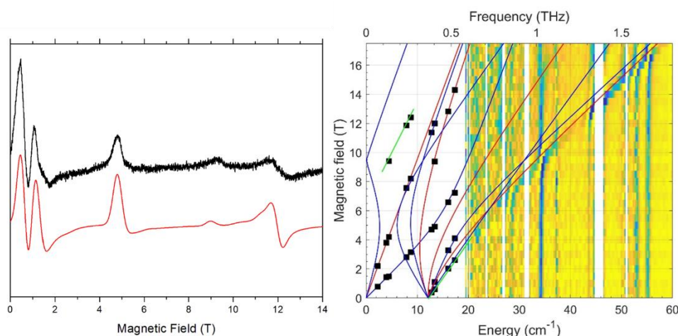
Figure 8. EPR spectrum of 1 as a pellet at 10 K and 402 GHz (black trace) and its simulation (red trace) using |D| = 5.25 \text{ cm}^{-1} , |E| = 1.75 \text{ cm}^{-1} , g_{\text{iso}} = 2.4 (left). Field vs. frequency dependence of EPR turning points in 1 (squares) along with simulations using |D| = 5.25 \text{ cm}^{-1} , |E| = 1.75 \text{ cm}^{-1} , g_{\text{iso}} = 2.25 (right). Blue curves: turning points with magnetic field parallel to the Z-axis of the ZFS tensor; red curves: B 0 parallel to Y-axis; green curves: off-axis turning points. The color plot of FIRMS data is described in the next section.
