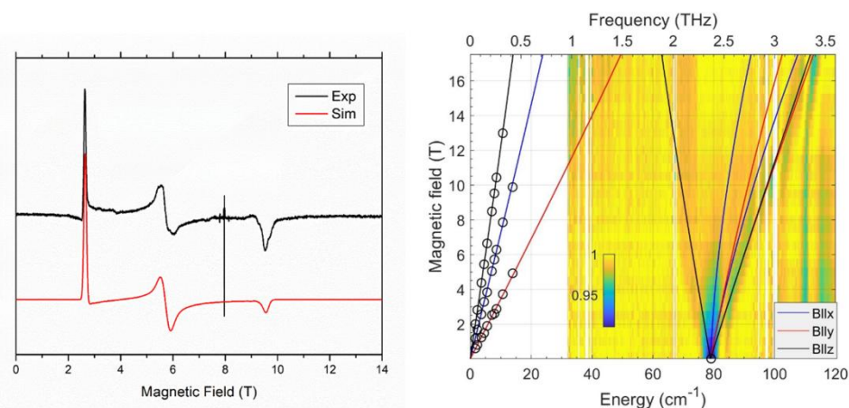
Figure 9. (Left) EPR spectrum of 5 as a pellet at 4.5 K and 237 GHz (black trace) and its simulation (red trace) using D = +36.36 \text{ cm}^{-1} , E = +8.97 \text{ cm}^{-1} , g_x = g_y = 2.44 and g_z = 2.16 . A group of narrow resonances near 7.95 T ( g = 2.12 ) is due to unidentified impurities. (Right) Experimental 2-D (magnetic field vs. energy) contour maps of FIRMS response of the same complex. HFEPR-observed turning points of the intra-Kramers transition are included as circles. The colour scales the field-induced changes in the transmission spectrum. The most intense change is observed at 80 \text{ cm}^{-1} in zero field. Lines are simulation of the EPR turning points. Other FIRMS data are shown in the Fig S7.
