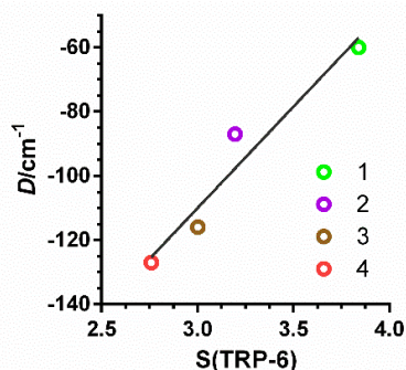
Figure 7. Plot of the axial anisotropy parameter versus the continuous symmetry measures parameter for the TPR-6 complexes 1-4 . The black solid line represents the best linear fitting leading to the equation D = 63 \cdot S(\text{TPR-6}) - 300 .
