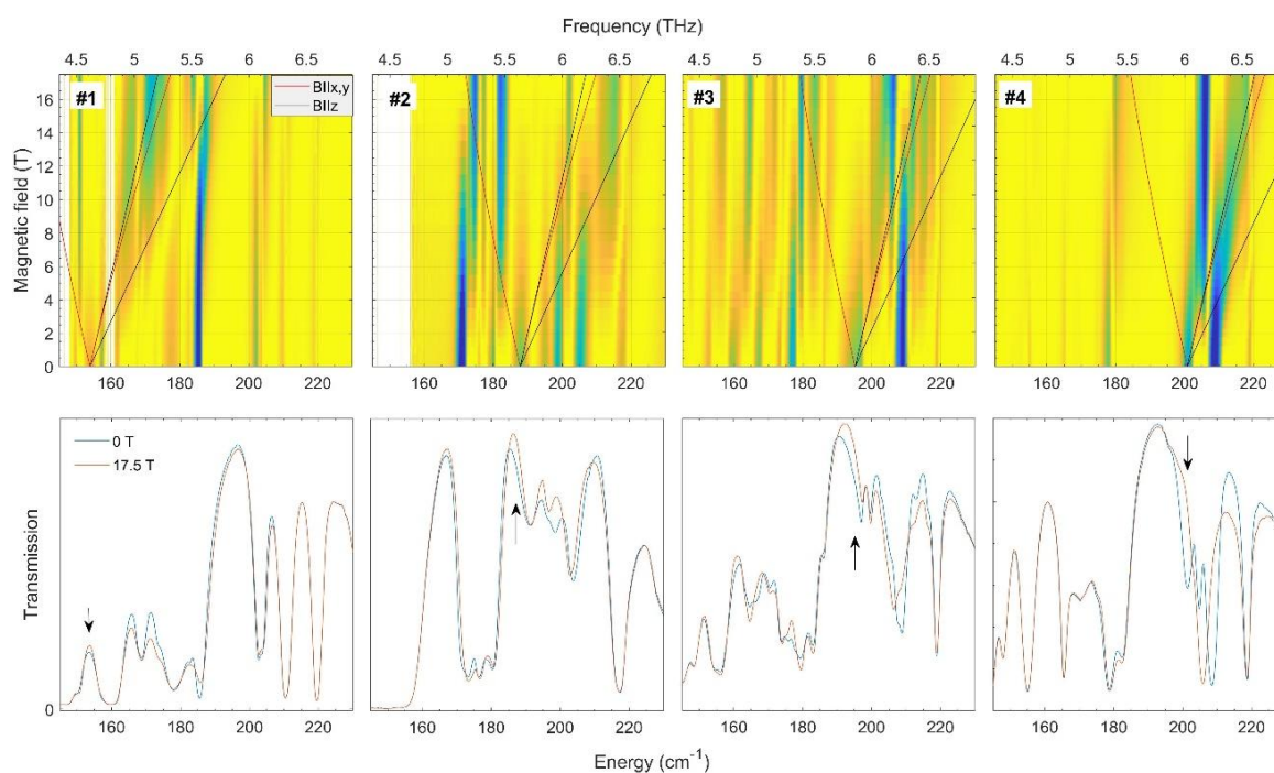
Figure 10. (Top) Experimental 2-D (magnetic field vs. energy) contour maps of FIRMS response for complexes 1-4 . Regions marked in blue represent resonance absorption that is sensitive to changing magnetic field. Regions in yellow are insensitive to the field. The lines are simulations of turning points for spin Hamiltonian, using a S=3/2 , the extracted 2D^* values, g_{iso} = 2.4 and E = 0 (they are only guidelines to illustrate how the energies of magnetic absorption are spreading in the applied magnetic field). (Bottom) Transmission spectra recorded on powder pellet of the complexes at T = 4.2 K and at the indicated magnetic fields. Arrows indicate the 2D^* positions suggested for these compounds.
