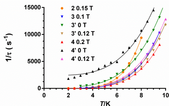
Figure 14. – Temperature dependence of the inverse of the relaxation times for the indicated compounds and magnetic fields. Solid lines represent the best fits to the relaxation processes specified in the text.
