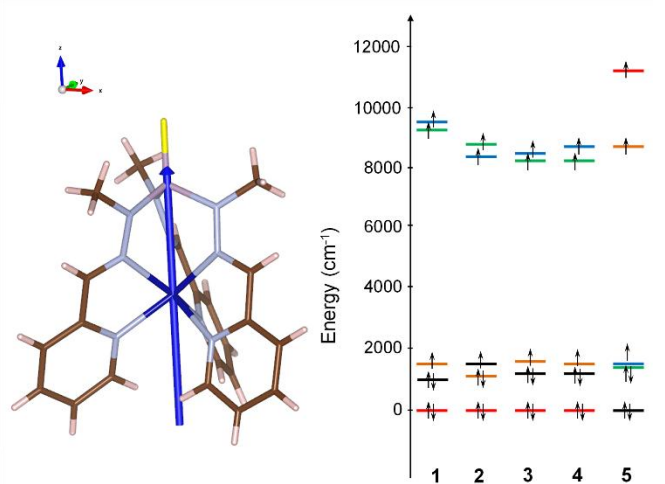
Figure 11.- Orientation of the axial anisotropy axis of compound 2 , which almost coincides with the pseudo C_3 axis of the molecule (left). NEVPT2-AILFT computed d-orbital energy diagram for complexes 1-5 (right). Colours code: d_{z^2} (red), d_{x^2-y^2} (orange), d_{xy} (black), d_{xz} (blue), d_{yz} (green).
