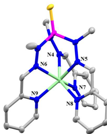
Figure 1: Perspective view of the molecular structure of 3 . Hydrogen atoms, perchlorate anions and solvent molecules are omitted for clarity. Only the \Delta enantiomer is given in this Figure.
