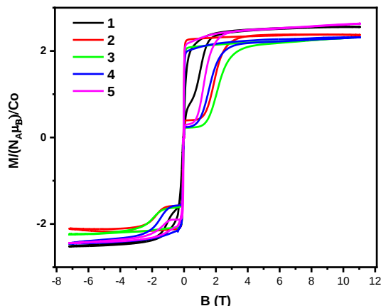
Figure 15. Pulse-field magnetization curves per cobalt atom for 1-5 at 0.4 K and a sweep rate of 4.10 T/ms.
