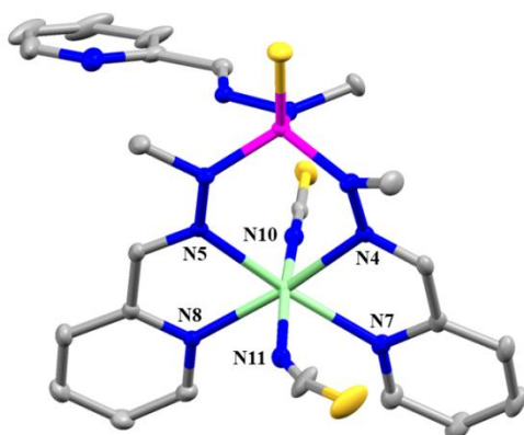
Figure 2: Perspective view of the molecular structure of compound 5 . Hydrogen atoms are omitted for clarity.
