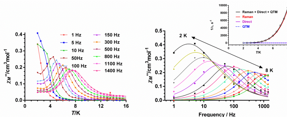
Figure 12. Temperature dependence of \chi''_M at different frequencies (left) and frequency dependence at different temperatures (right) for 2 under a field of 0.12 T. Contribution of each relaxation process to the slow relaxation of the magnetization (insert).
