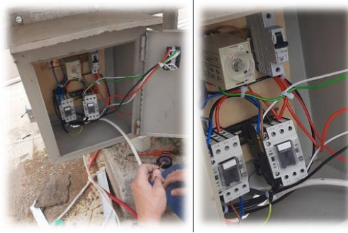
Figure 12 - Control unit utilized in the pilot project.
