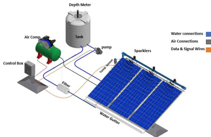
Figure 9 - Solar panel intelligent cleaning system, 3D CAD model
